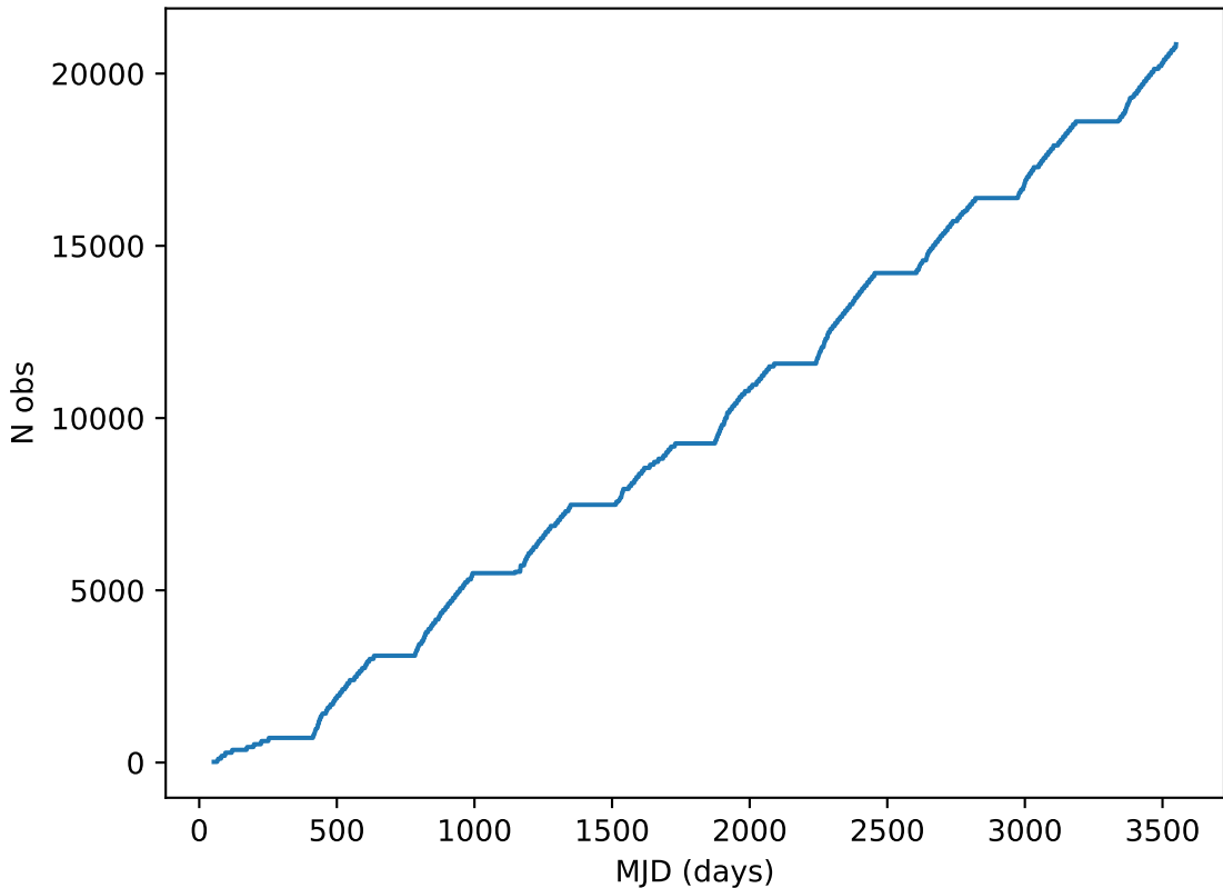
reweight_bulge_v3.3_10yrs note like DD:ELAISS1%: Cumulative
