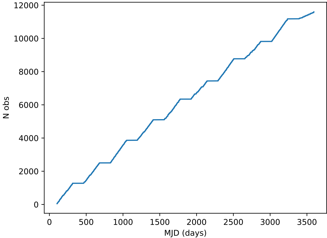
reweight_bulge_v3.3_10yrs note like DD:EDFS_b%: Cumulative
