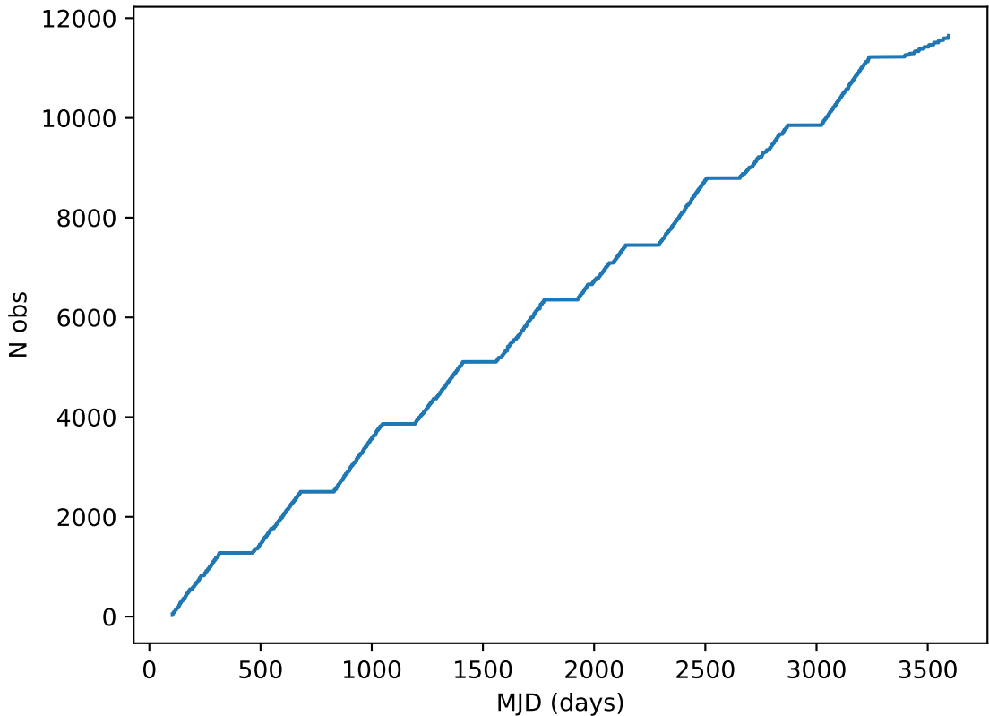
reweight_bulge_v3.3_10yrs note like DD:EDFS_a%: Cumulative
