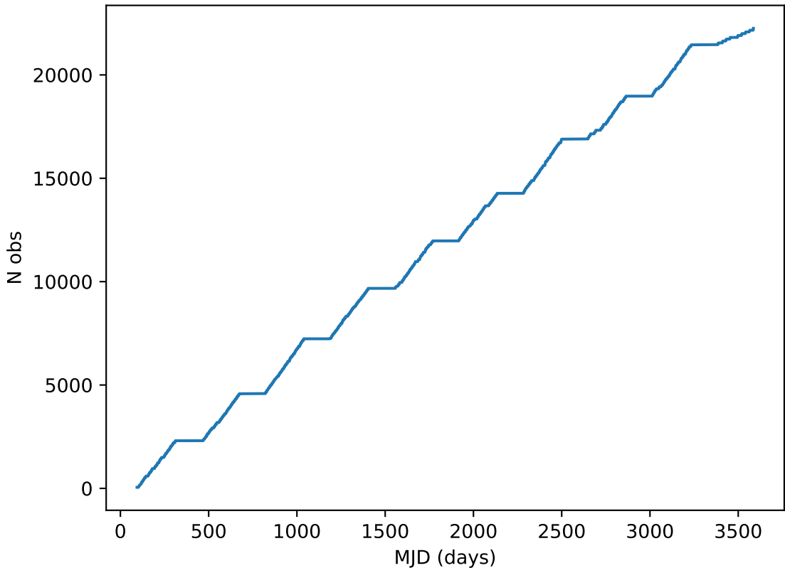
reweight_bulge_v3.3_10yrs note like DD:ECDFS%: Cumulative
