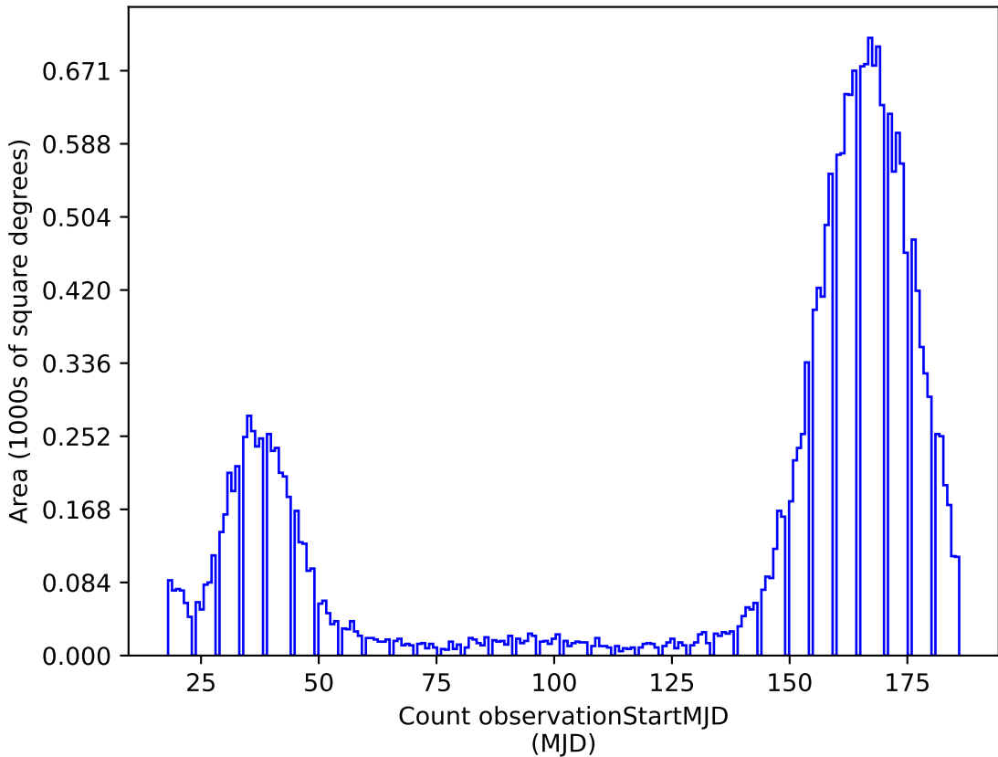
reweight_bulge_v3.3_10yrs y: Count observationStartMJD
