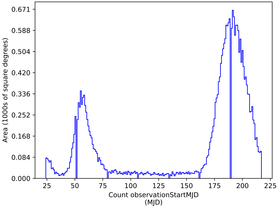
reweight_bulge_v3.3_10yrs i: Count observationStartMJD
