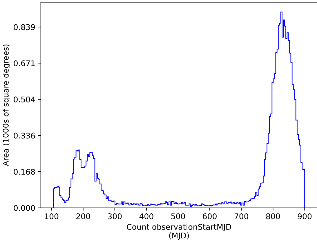
reweight_bulge_v3.3_10yrs : Count observationStartMJD
