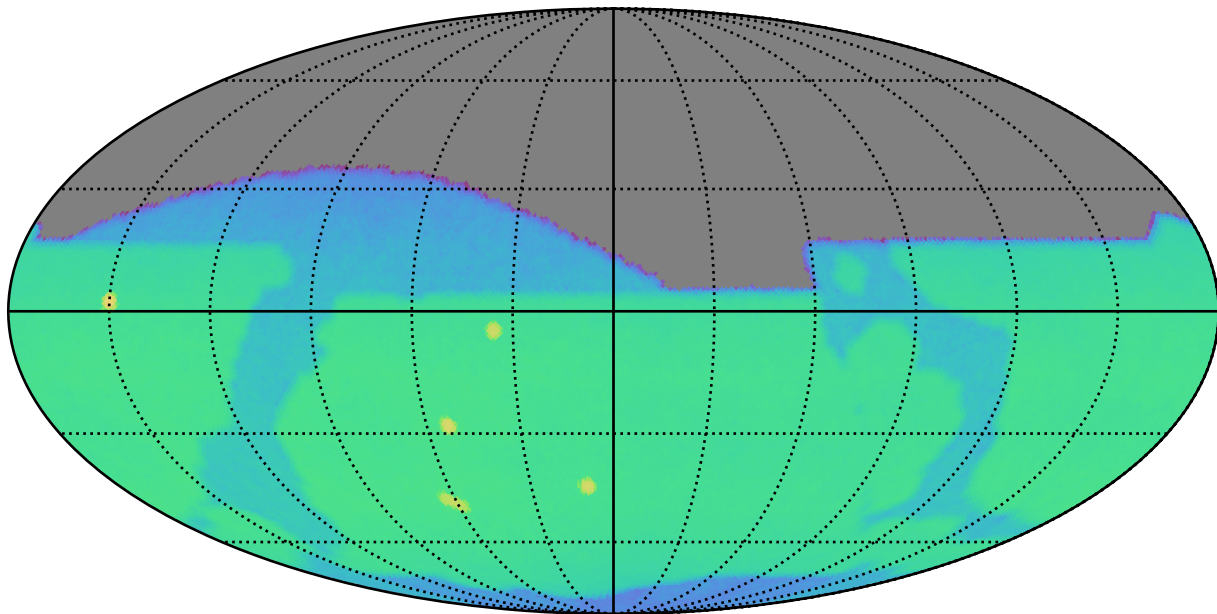
reweight_bulge_v3.3_10yrs z: CoaddM5
