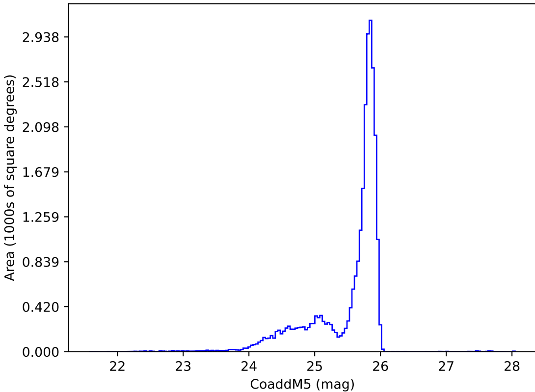
reweight_bulge_v3.3_10yrs z: CoaddM5
