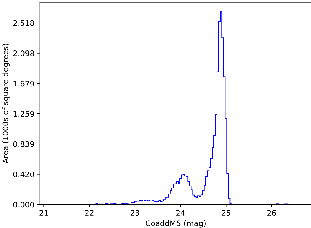
reweight_bulge_v3.3_10yrs y: CoaddM5
