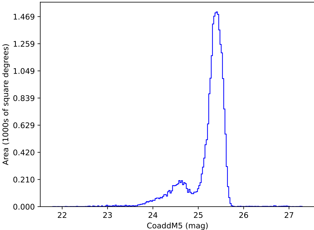
reweight_bulge_v3.3_10yrs u: CoaddM5
