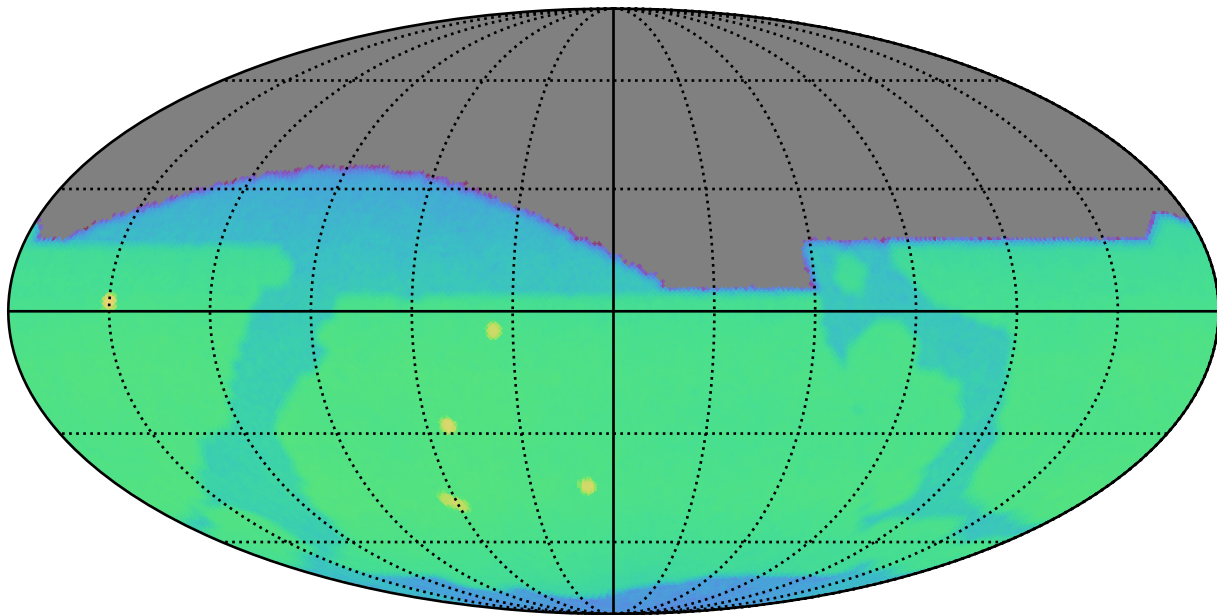
reweight_bulge_v3.3_10yrs i: CoaddM5
