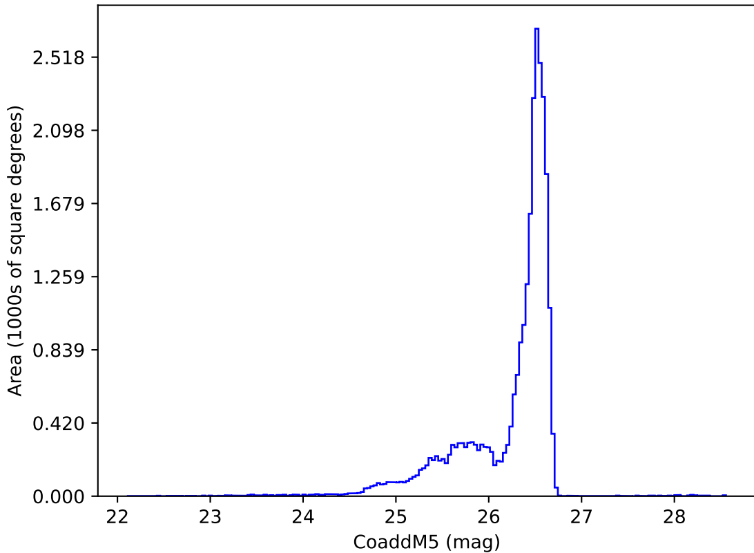
reweight_bulge_v3.3_10yrs i: CoaddM5
