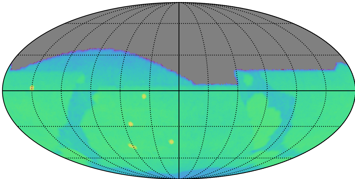
reweight_bulge_v3.3_10yrs g: CoaddM5
