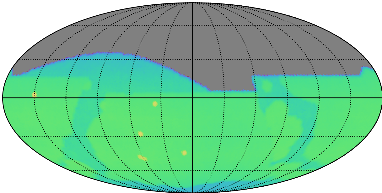
reweight_bulge_v3.3_10yrs : CoaddM5
