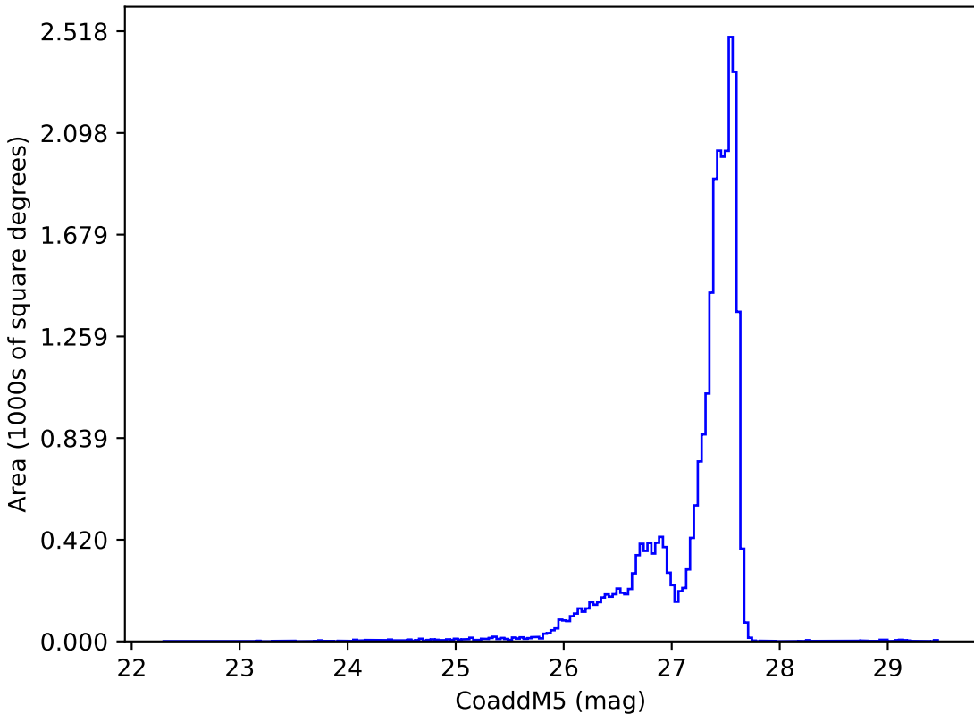
reweight_bulge_v3.3_10yrs : CoaddM5
