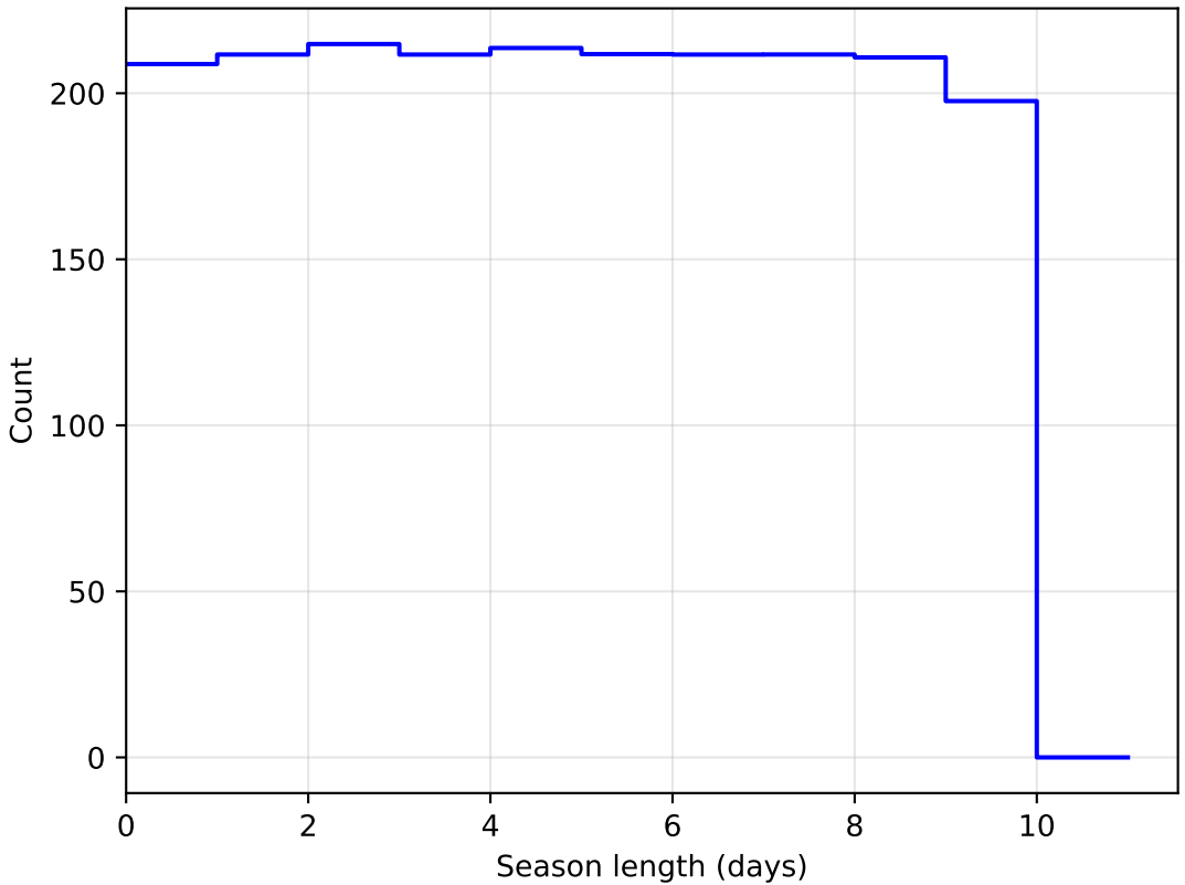
reweight_bulge_v3.3_10yrs DD:EDFS all bands: SeasonLength
