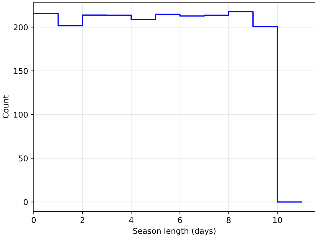
reweight_bulge_v3.3_10yrs DD:ECDFS all bands: SeasonLength
