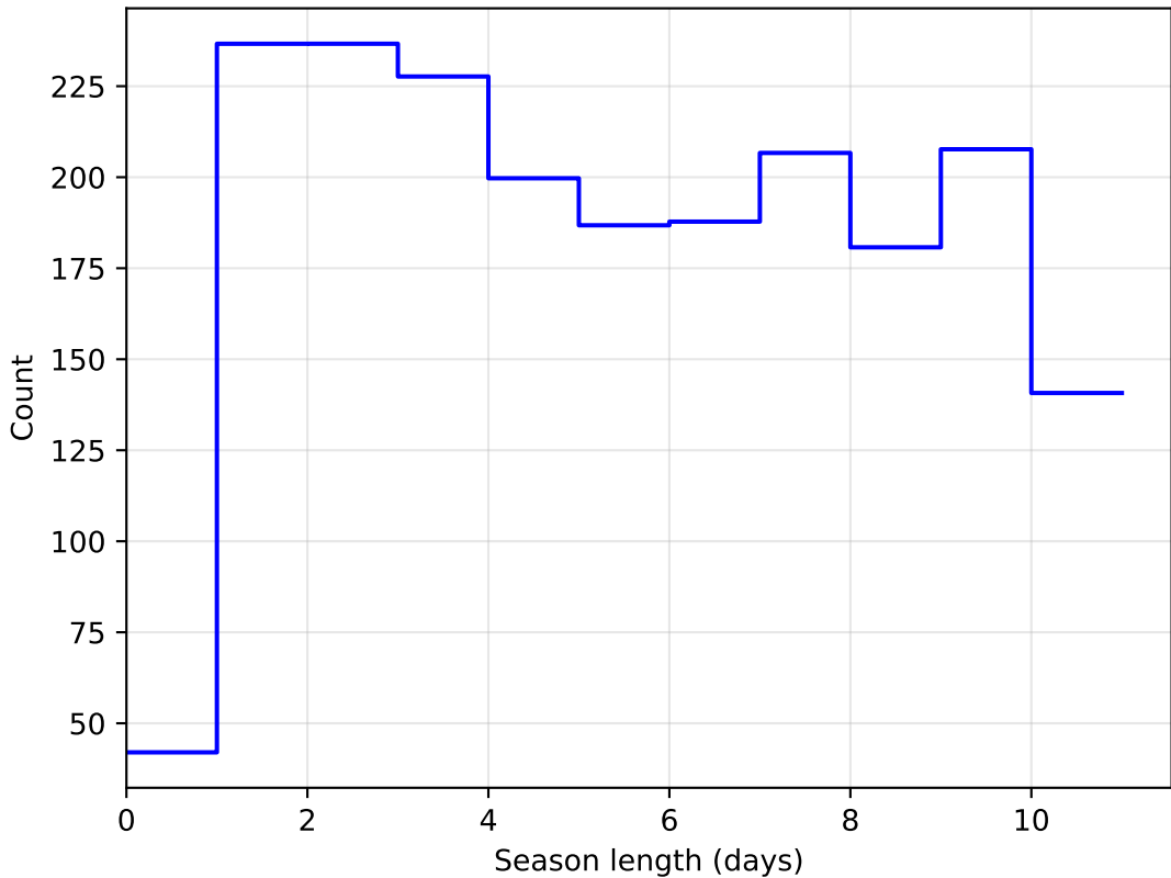
reweight_bulge_v3.3_10yrs DD: COSMOS all bands: SeasonLength
