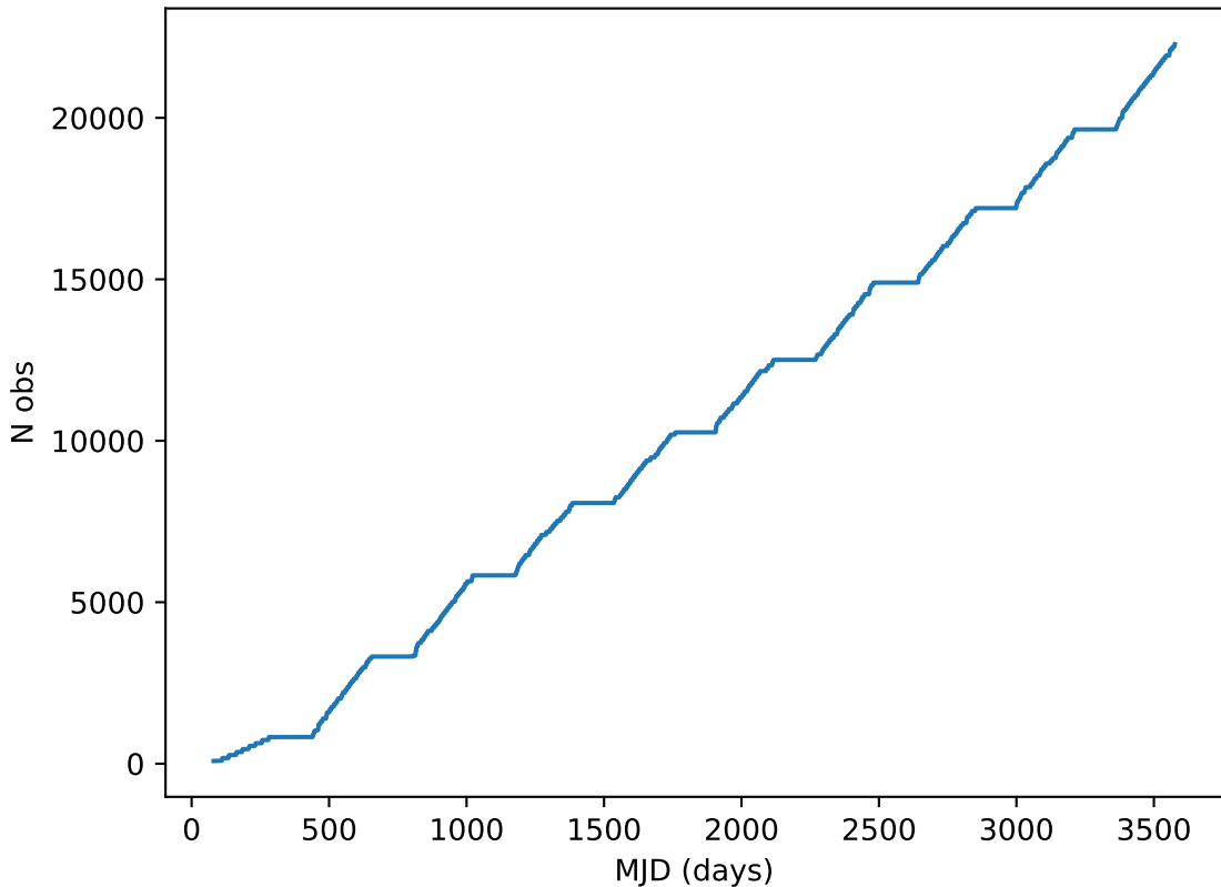
reweight_bulge_v3.3_10yrs all bands: DD:XMM_LSS Cumulative NVisits
