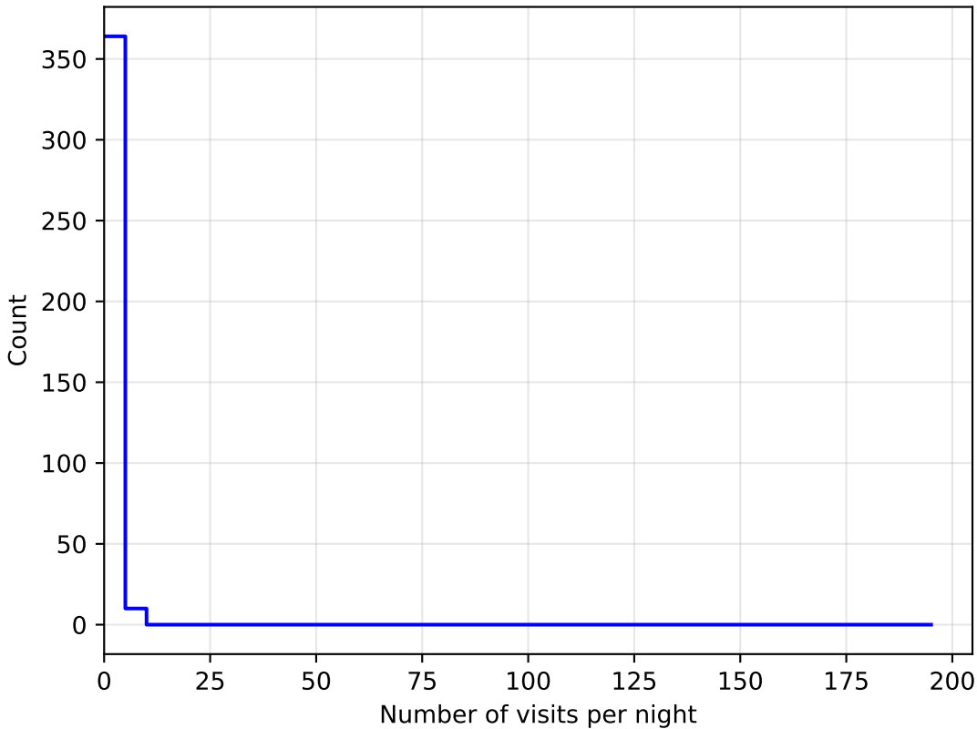
reweight_bulge_v3.3_10yrs all bands: DD:WFD NVisitsPerNight
