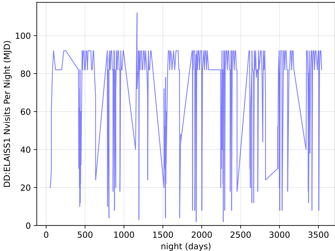
reweight_bulge_v3.3_10yrs all bands: DD:ELAISS1 Nvisits Per Night
