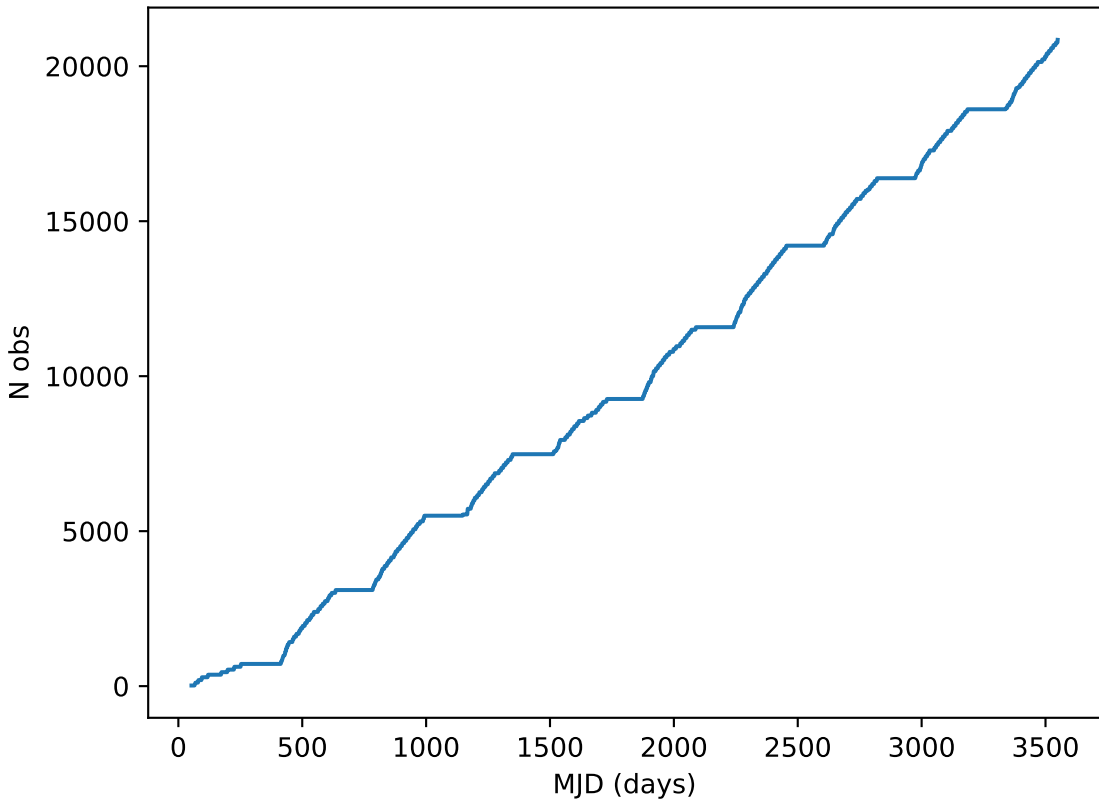
reweight_bulge_v3.3_10yrs all bands: DD:ELAISS1 Cumulative NVisits
