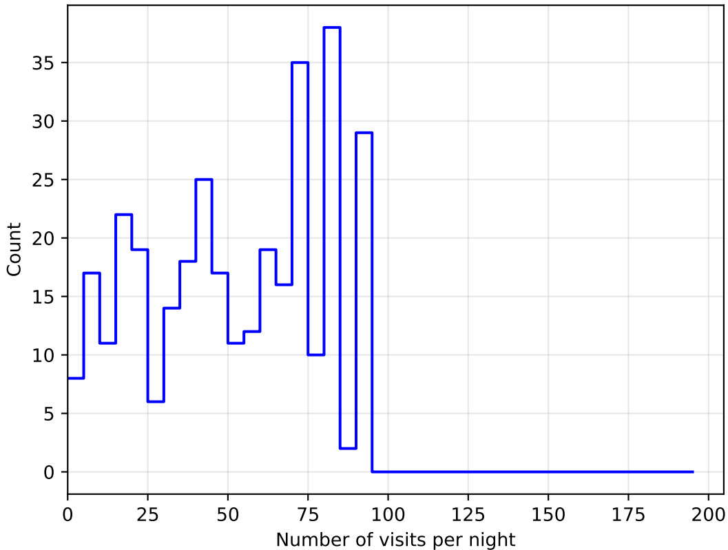
reweight_bulge_v3.3_10yrs all bands: DD:EDFS NVisitsPerNight
