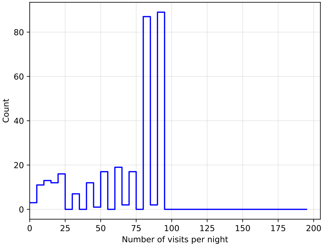
reweight_bulge_v3.3_10yrs all bands: DD:ECDFS NVisitsPerNight
