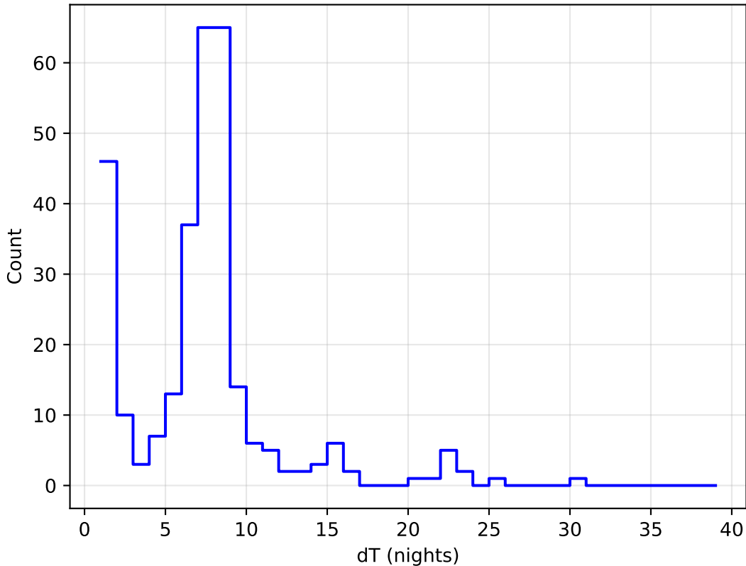
reweight_bulge_v3.3_10yrs all bands: DD:ECDFS Delta Nights Histogram
