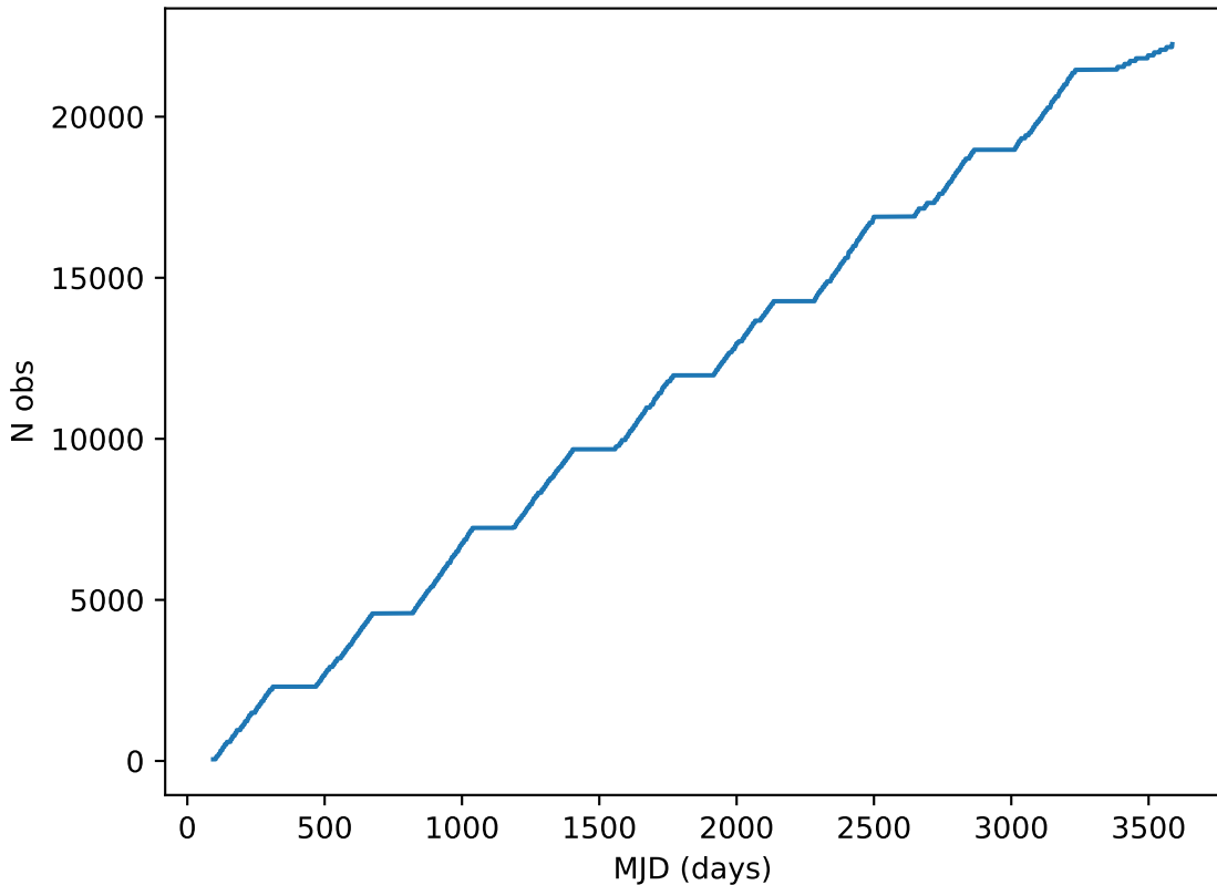
reweight_bulge_v3.3_10yrs all bands: DD:ECDFS Cumulative NVisits
