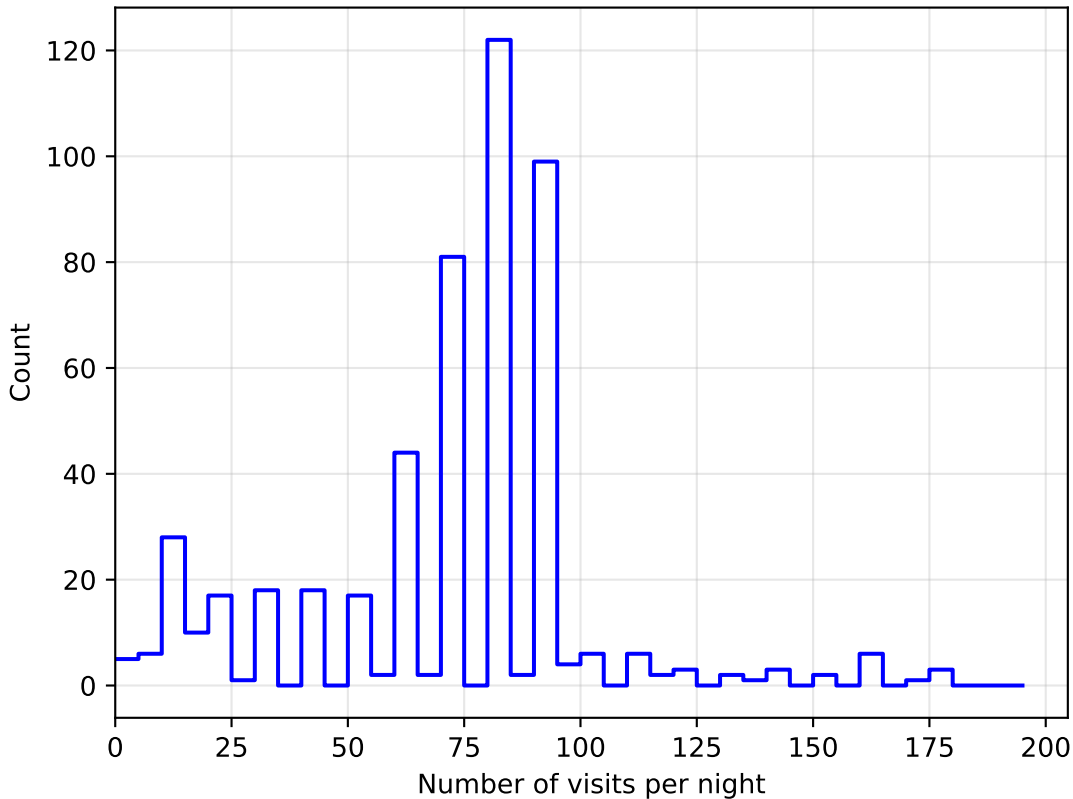
reweight_bulge_v3.3_10yrs all bands: DD:COSMOS NVisitsPerNight
