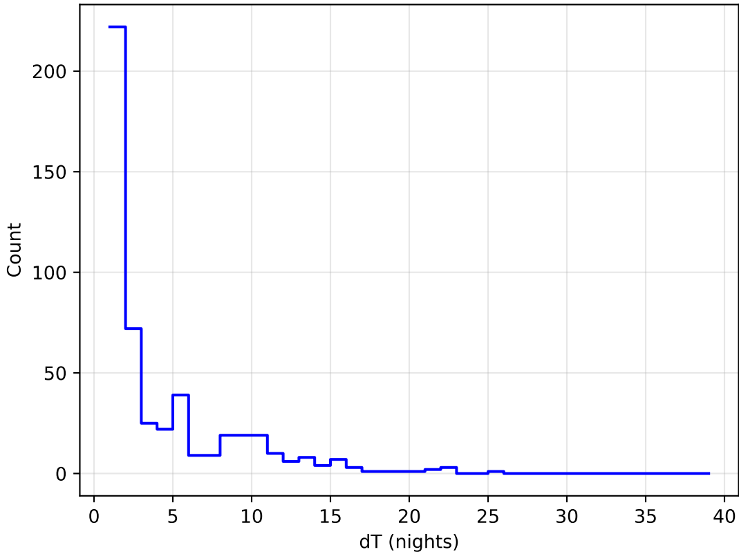
reweight_bulge_v3.3_10yrs all bands: DD: COSMOS Delta Nights Histogram
