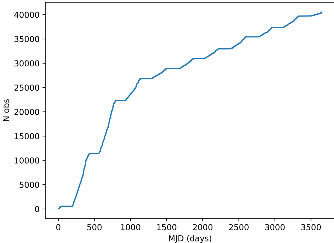
reweight_bulge_v3.3_10yrs all bands: DD:COSMOS Cumulative NVisits
