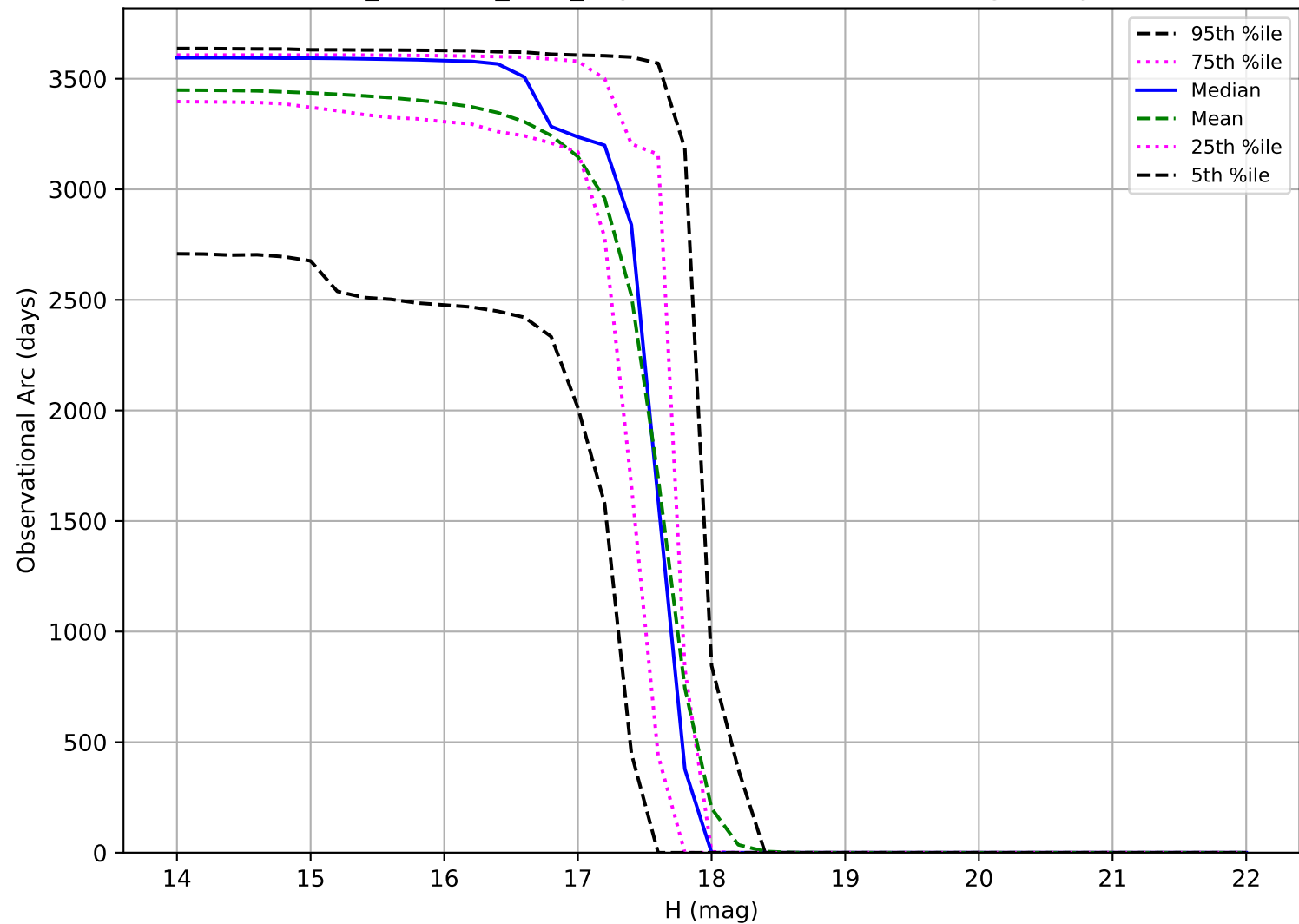
retro_baseline_v2.0_10yrs: Observational Arc Length Trojan
