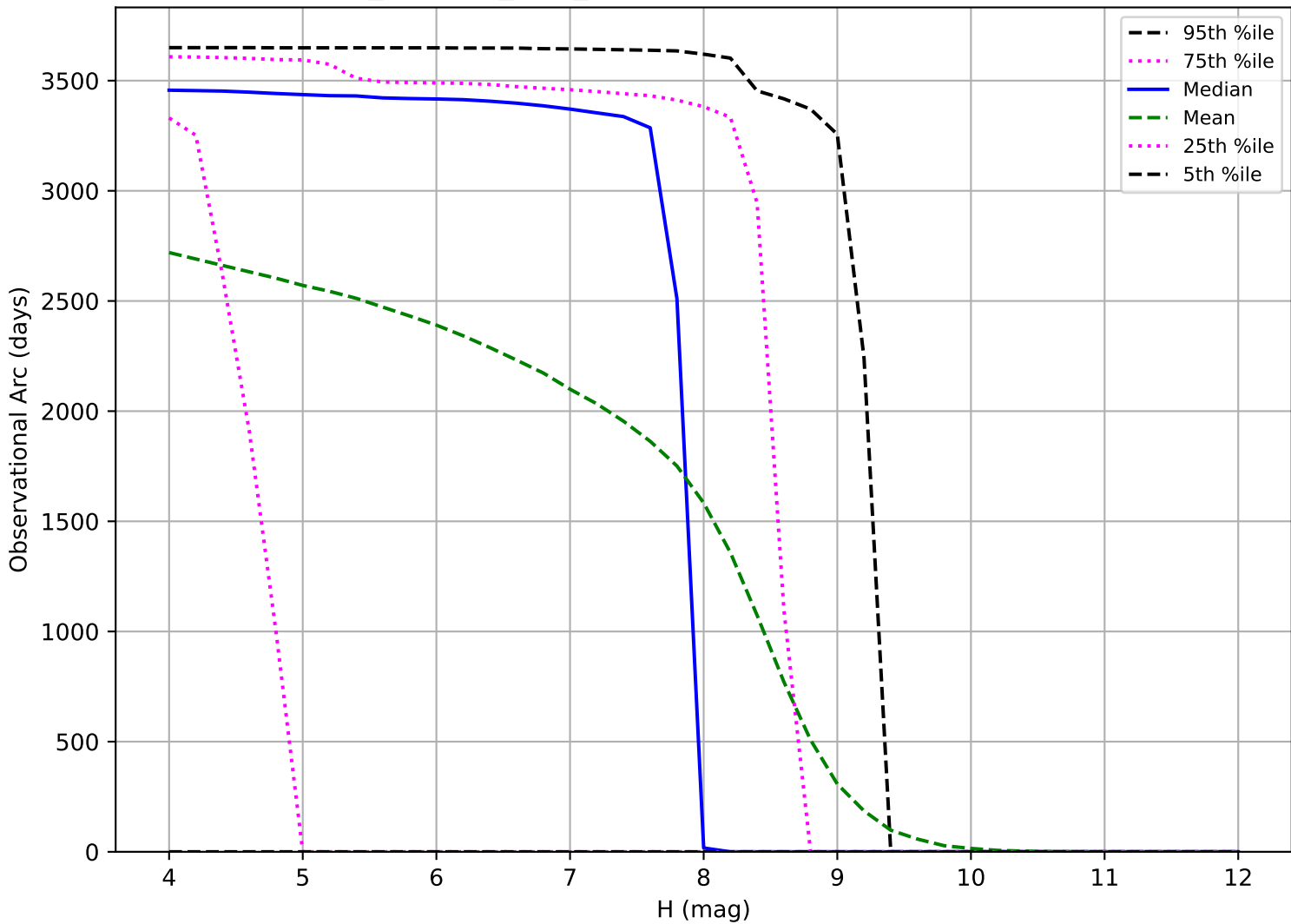
retro_baseline_v2.0_10yrs: Observational Arc Length TNO
