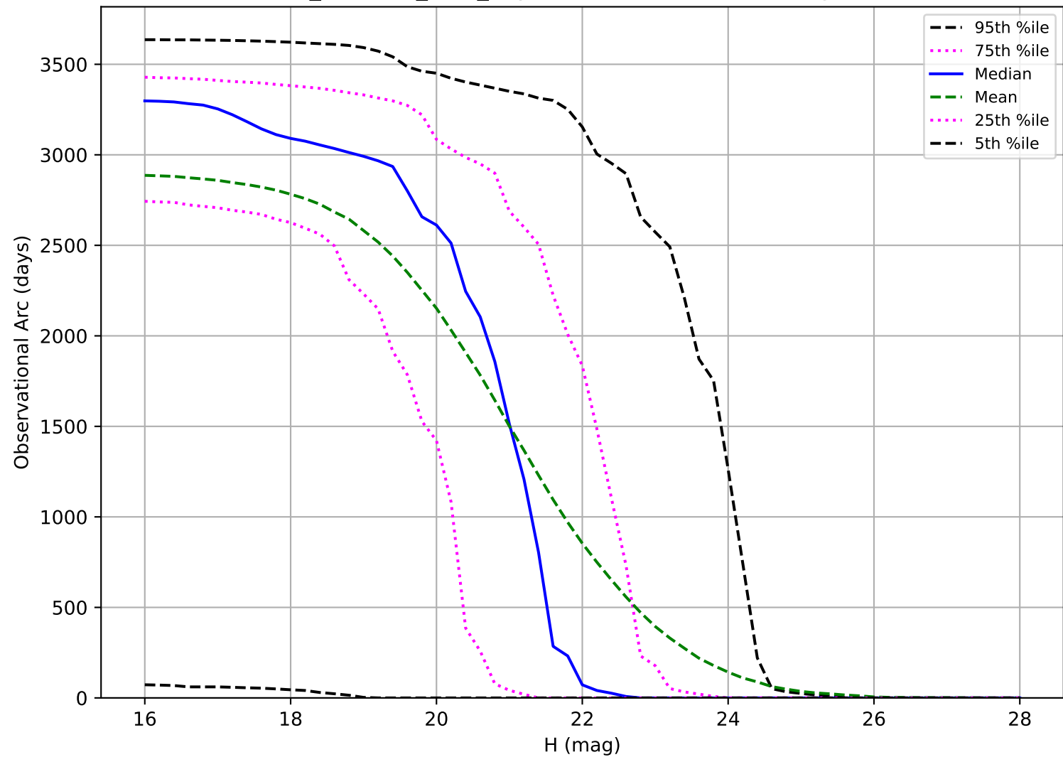
retro_baseline_v2.0_10yrs: Observational Arc Length PHA
