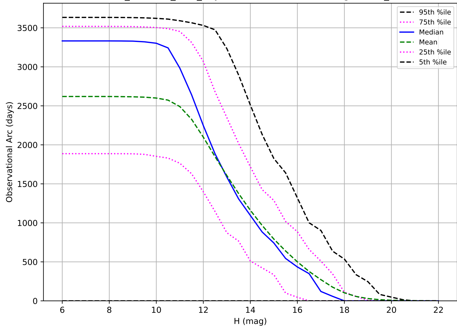
retro_baseline_v2.0_10yrs: Observational Arc Length OCC_r5
