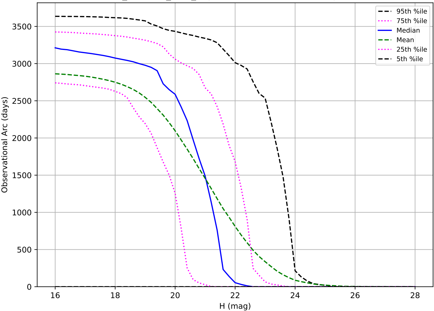
retro_baseline_v2.0_10yrs: Observational Arc Length NEO
