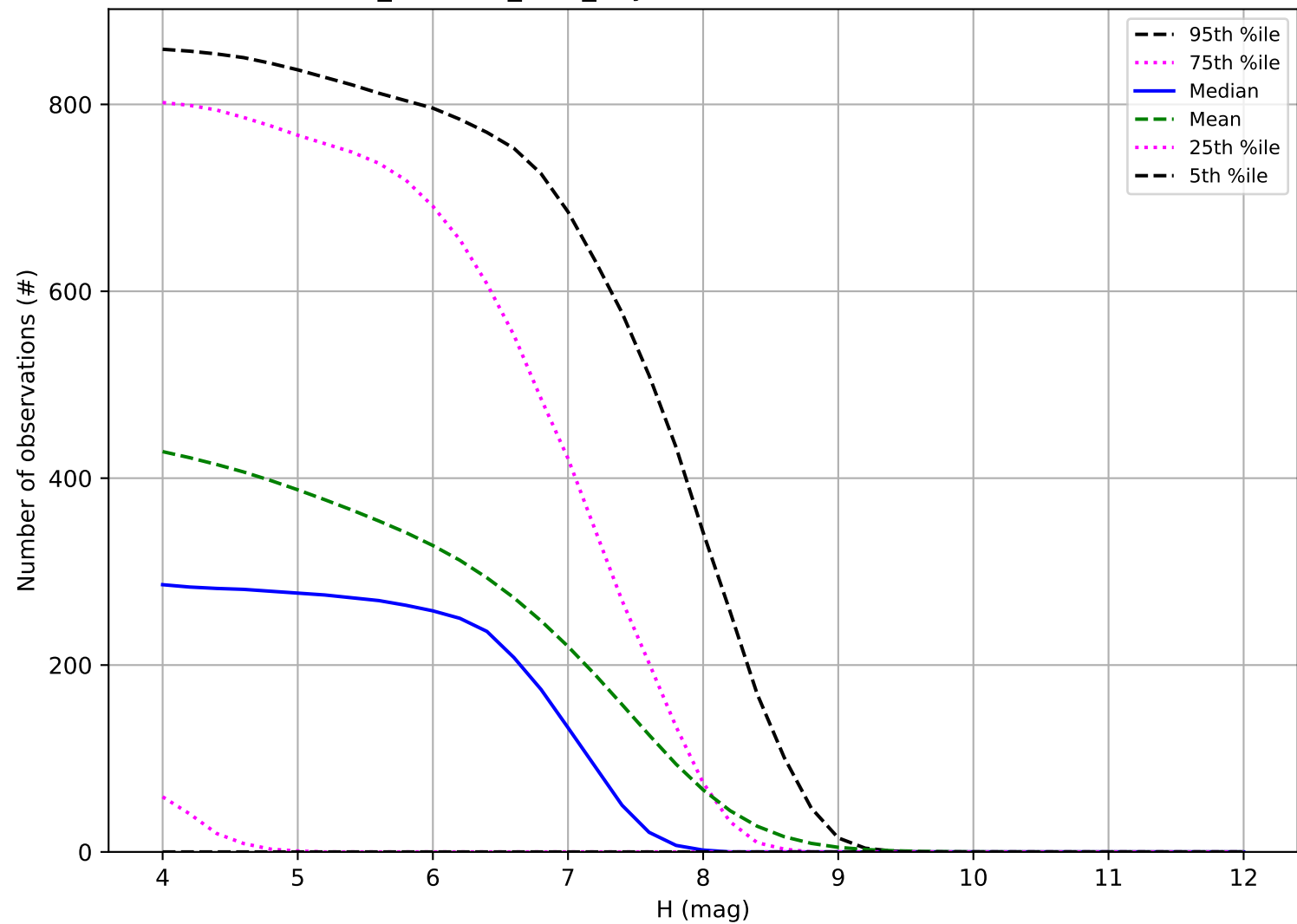
retro_baseline_v2.0_10yrs: Number of observations TNO
