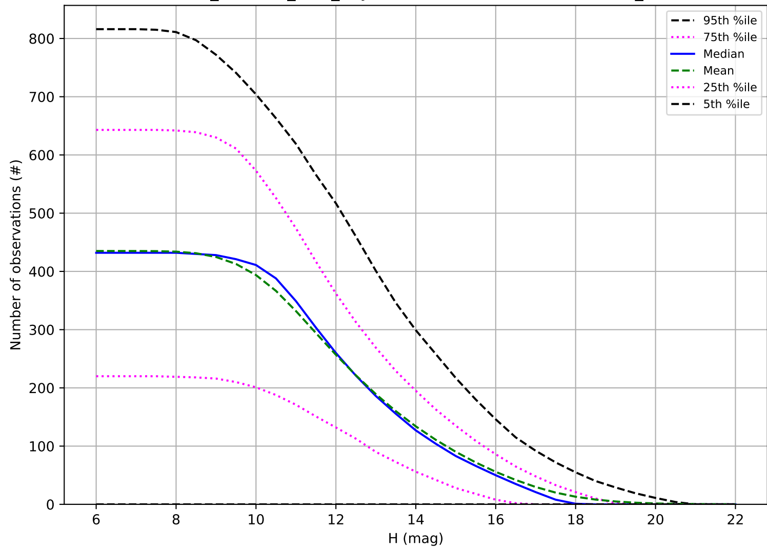
retro_baseline_v2.0_10yrs: Number of observations OCC_r5
