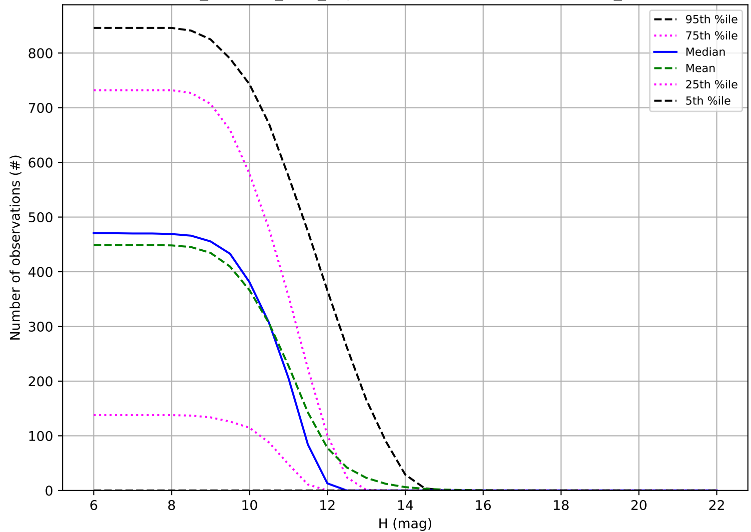
retro_baseline_v2.0_10yrs: Number of observations OCC_r20
