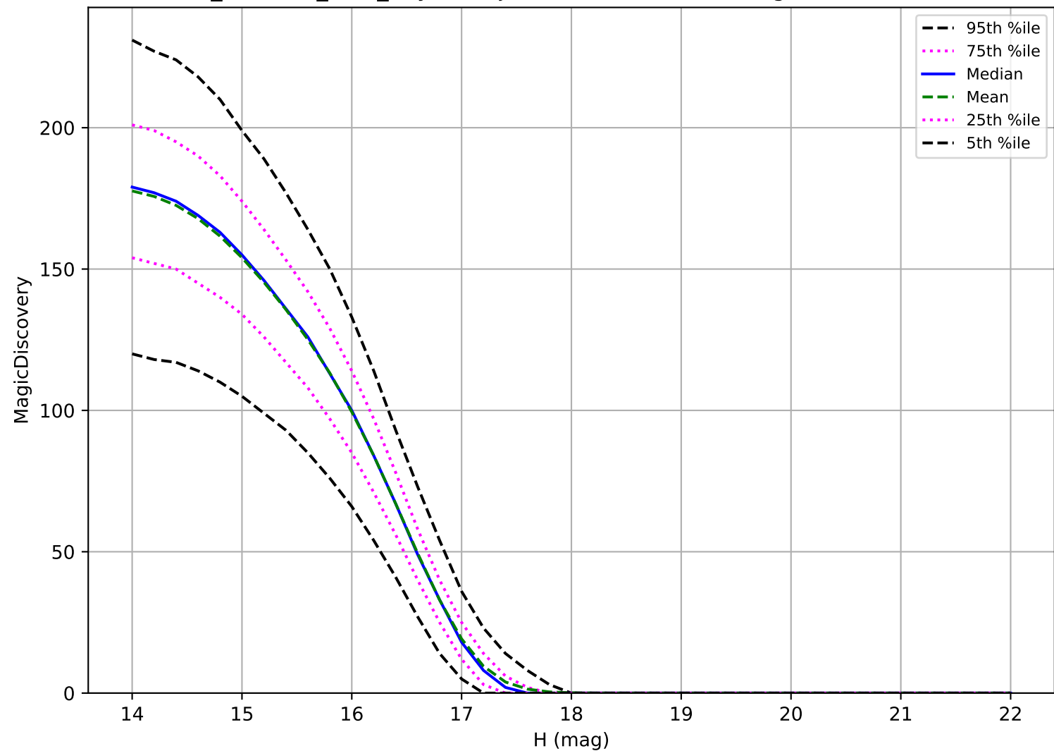
retro_baseline_v2.0_10yrs: Trojan 6 detections in 60 nights detection loss
