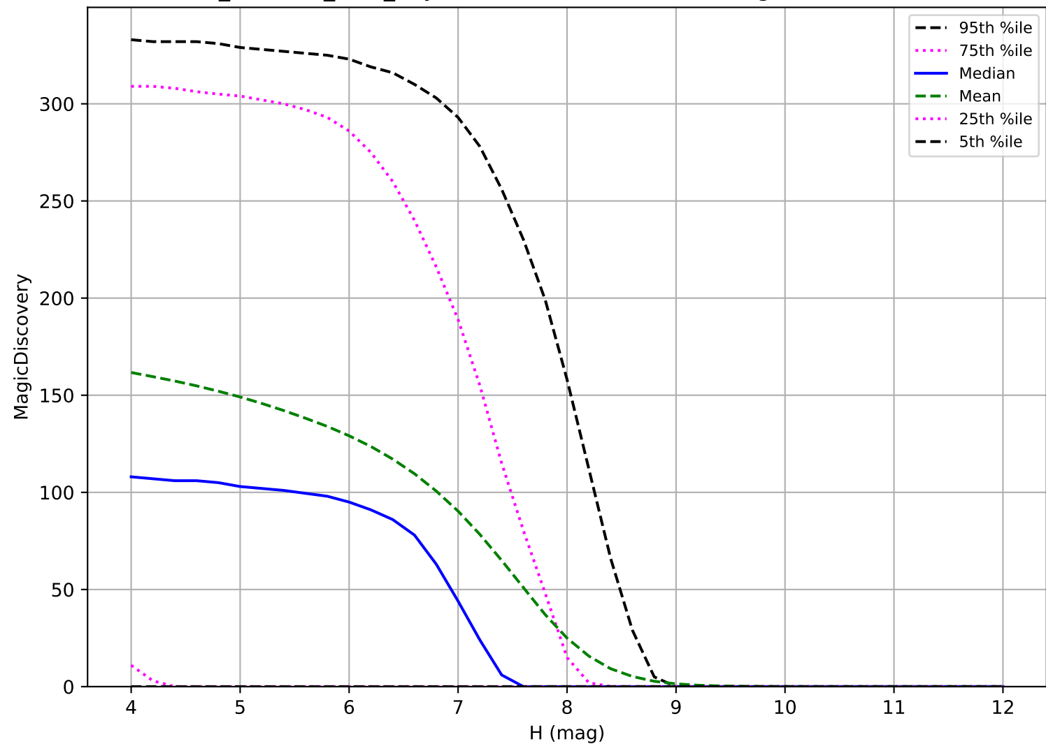
retro_baseline_v2.0_10yrs: TNO 6 detections in 60 nights detection loss
