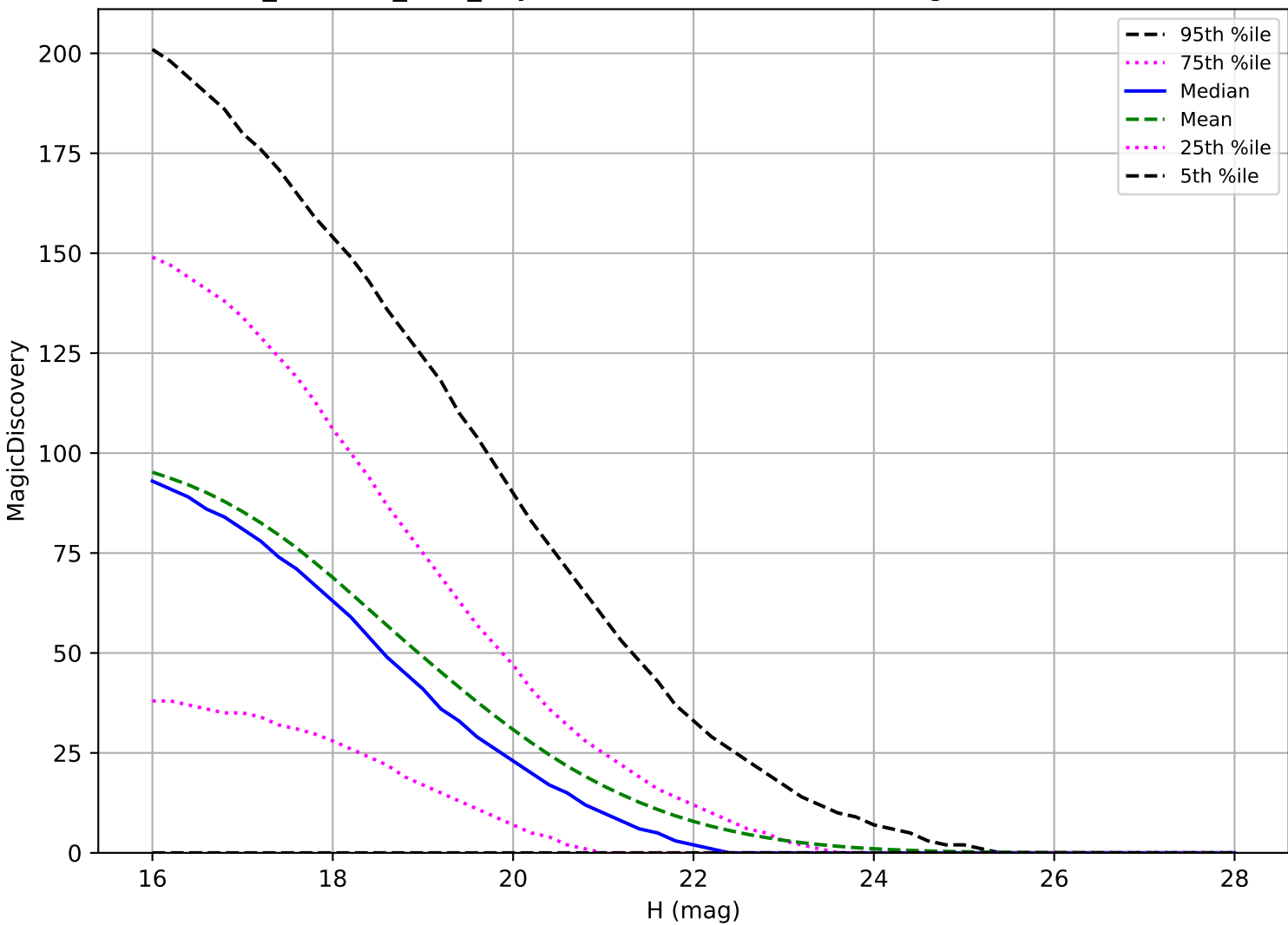
retro_baseline_v2.0_10yrs: PHA 6 detections in 60 nights detection loss
