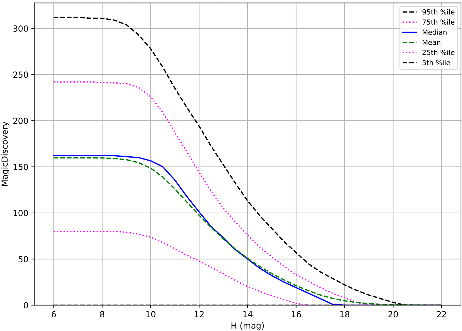
retro_baseline_v2.0_10yrs: OCC_r5 6 detections in 60 nights detection loss
