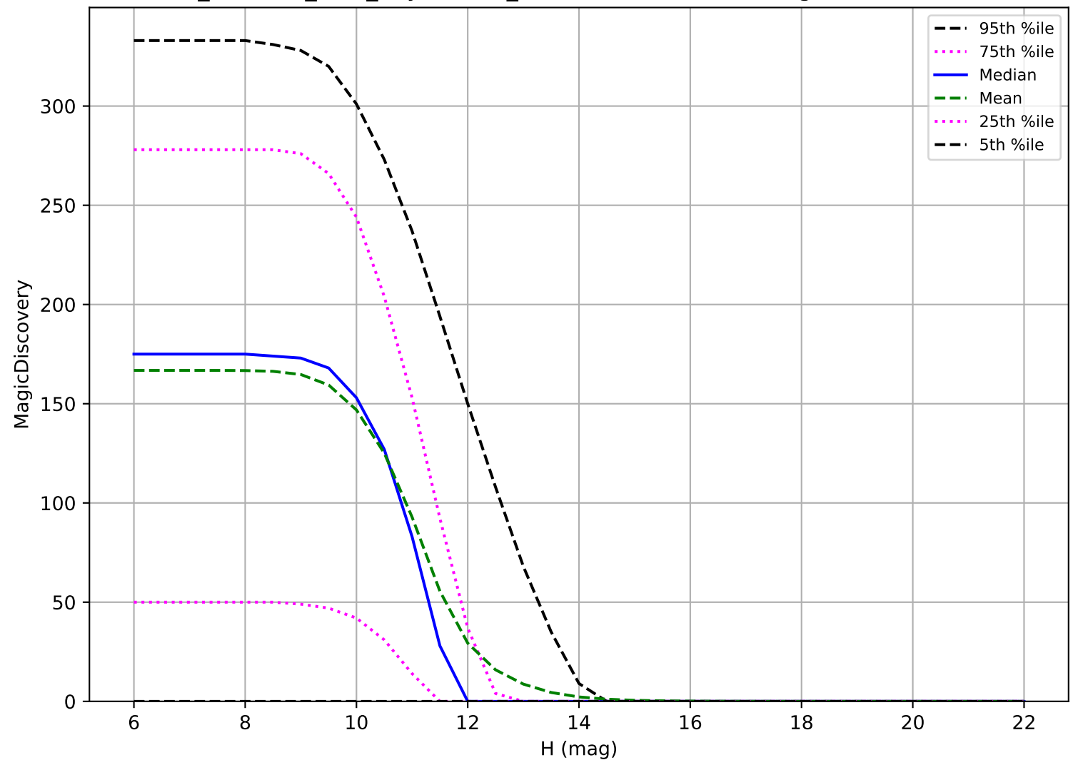
retro_baseline_v2.0_10yrs: OCC_r20 6 detections in 60 nights detection loss
