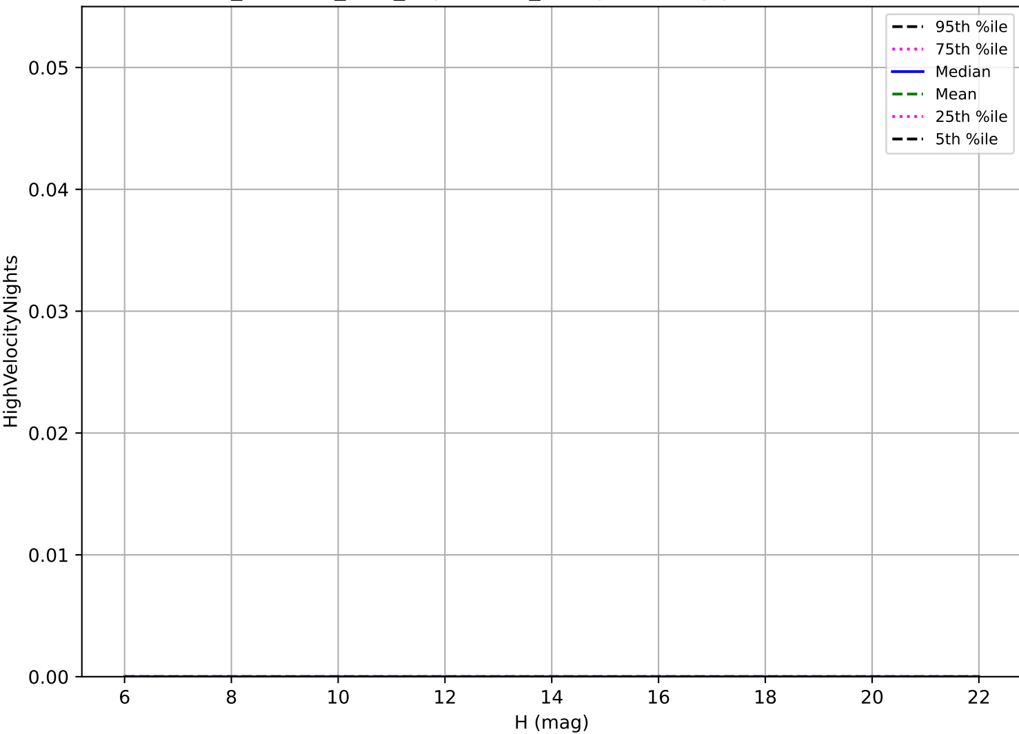
retro_baseline_v2.0_10yrs: OCC_r5 High velocity pair detection loss
