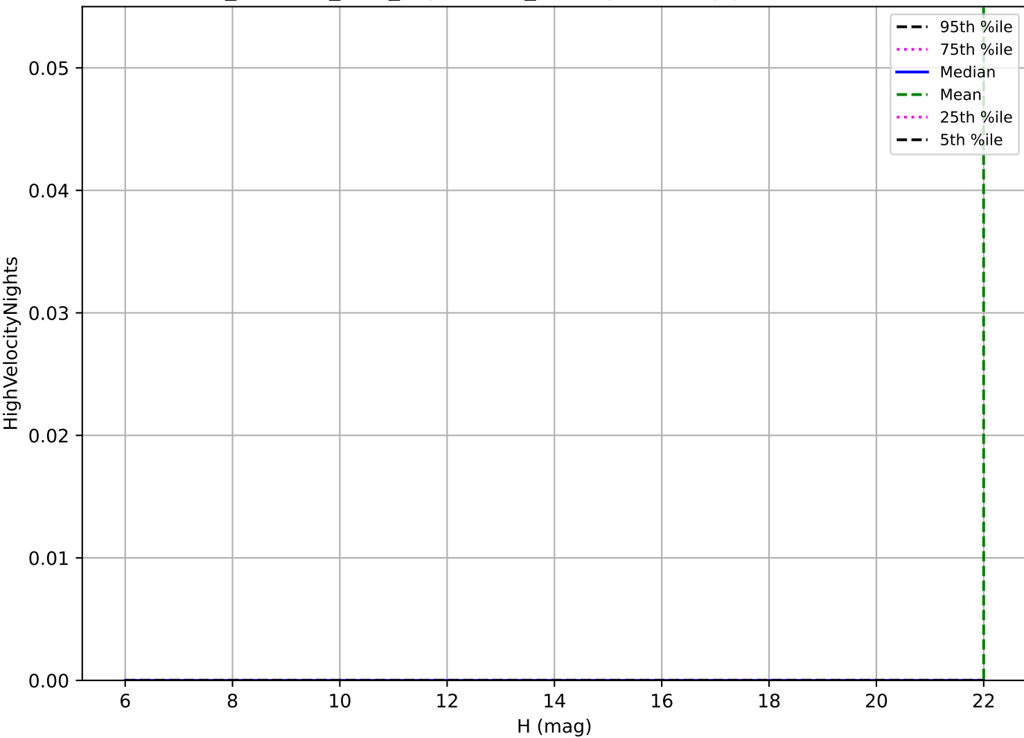
retro_baseline_v2.0_10yrs: OCC_r20 High velocity pair detection loss
