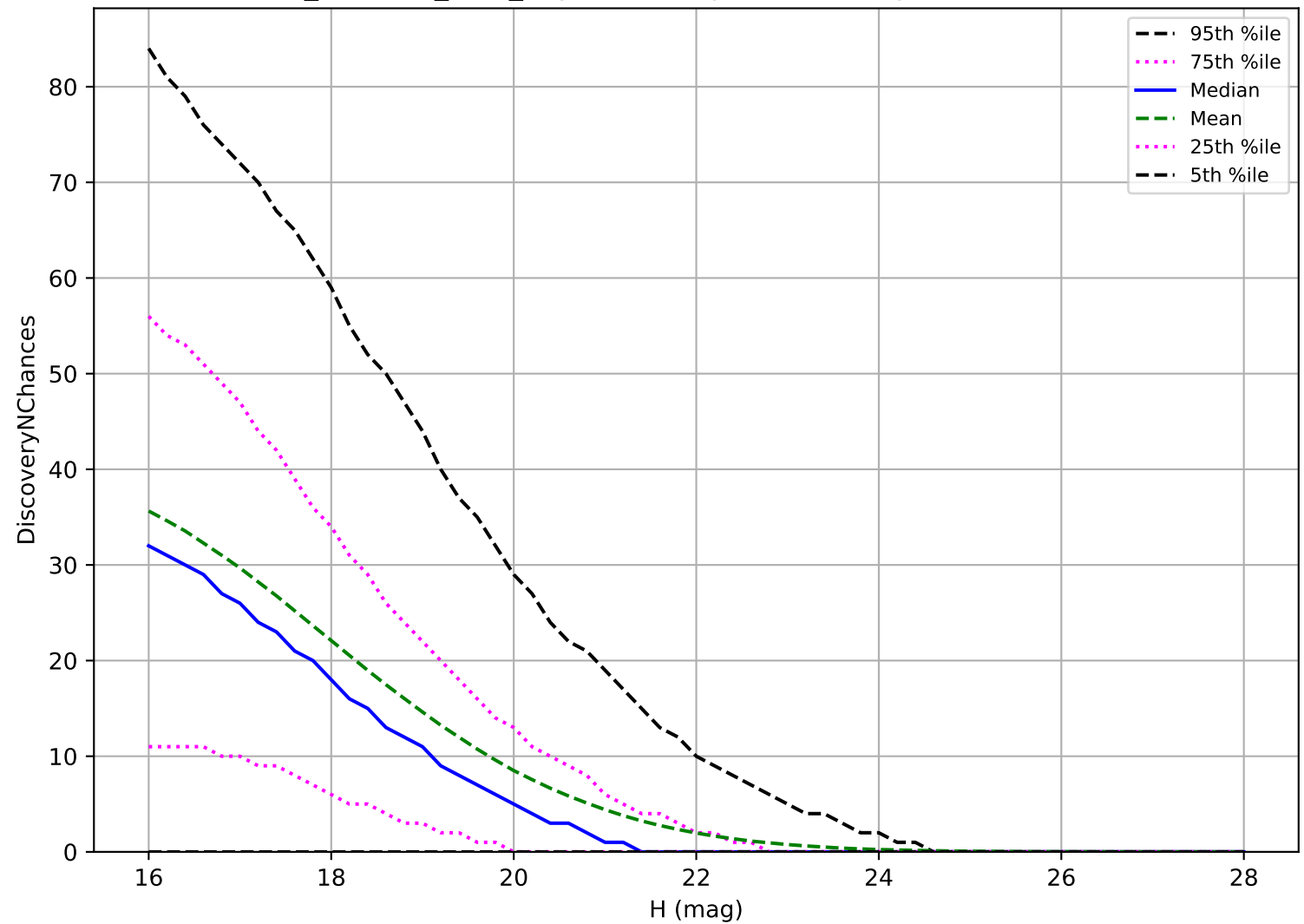
retro_baseline_v2.0_10yrs: PHA 3 pairs in 15 nights detection loss
