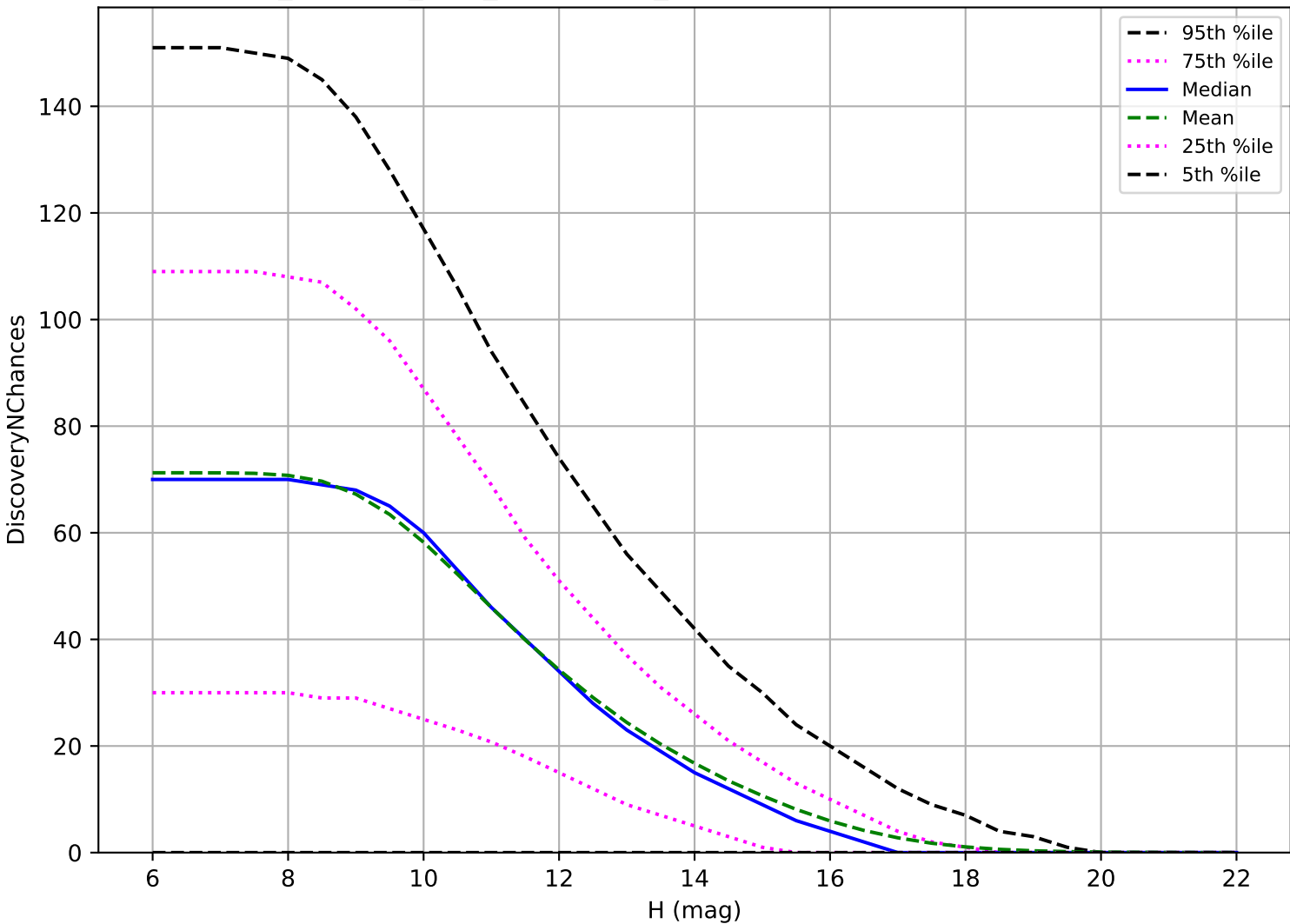
retro_baseline_v2.0_10yrs: OCC_r5 3 pairs in 15 nights detection loss
