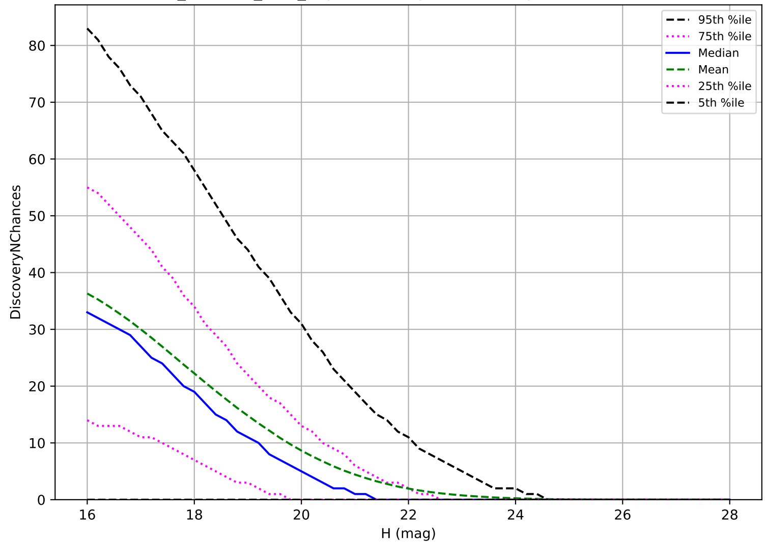
retro_baseline_v2.0_10yrs: NEO 3 pairs in 15 nights detection loss
