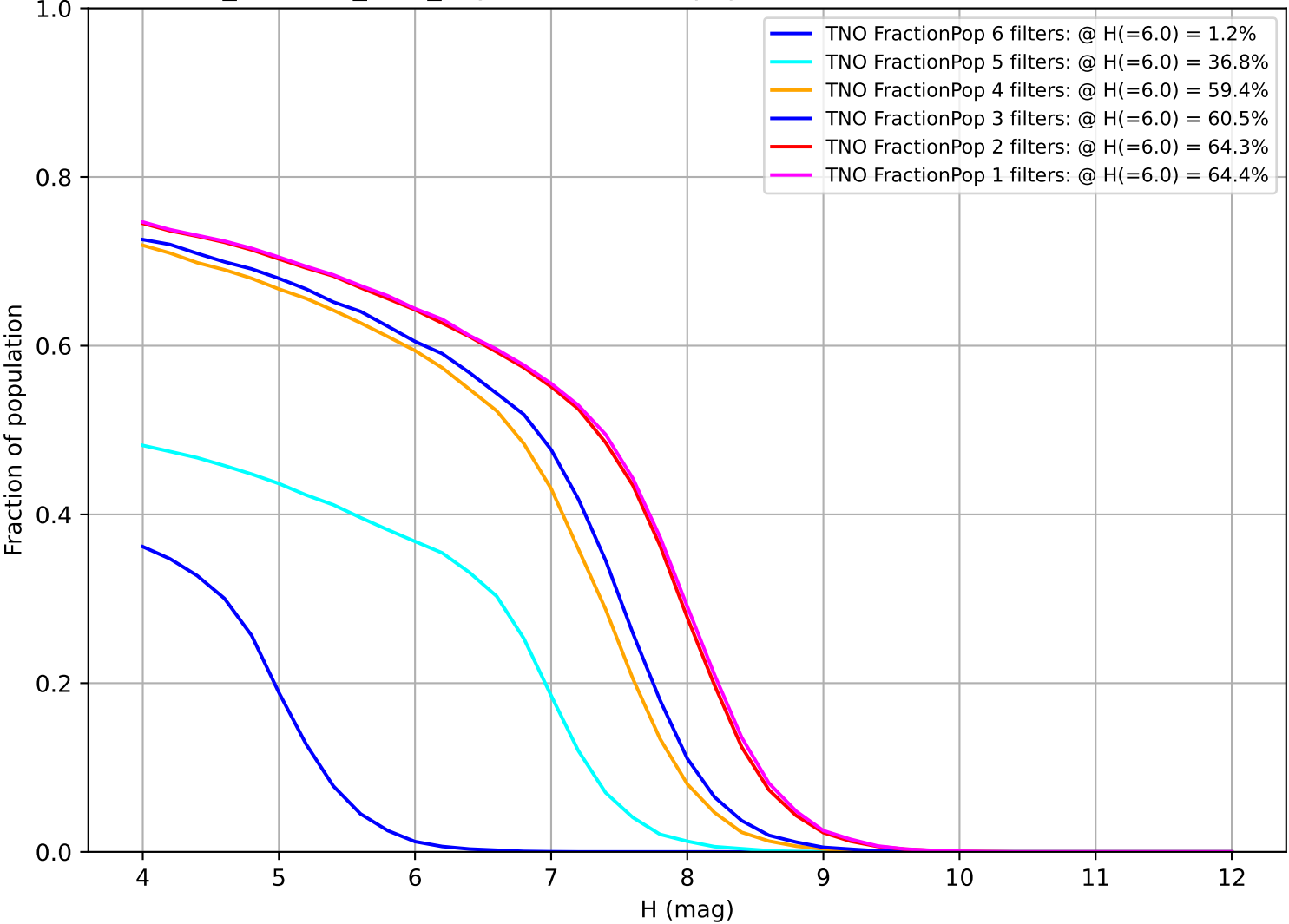
retro_baseline_v2.0_10yrs: Fraction of population with colors in X filters TNO
