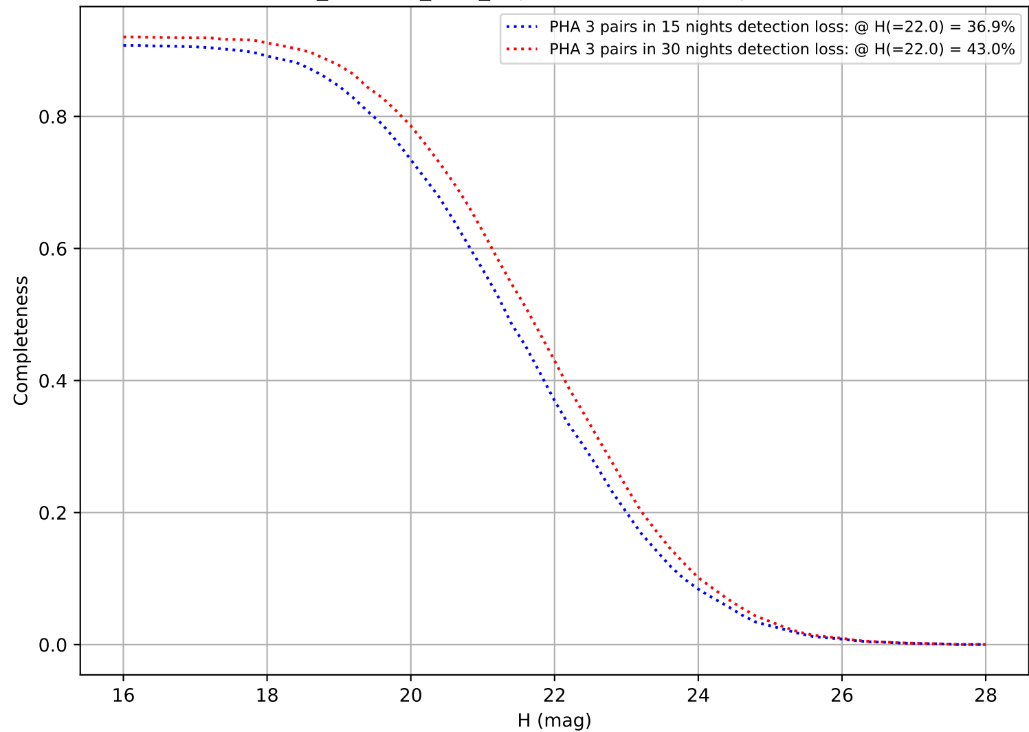
retro_baseline_v2.0_10yrs: DifferentialCompleteness
